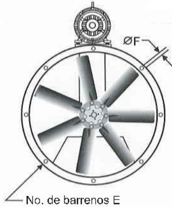
VISTA FRONTAL (FRONT VIEW)
